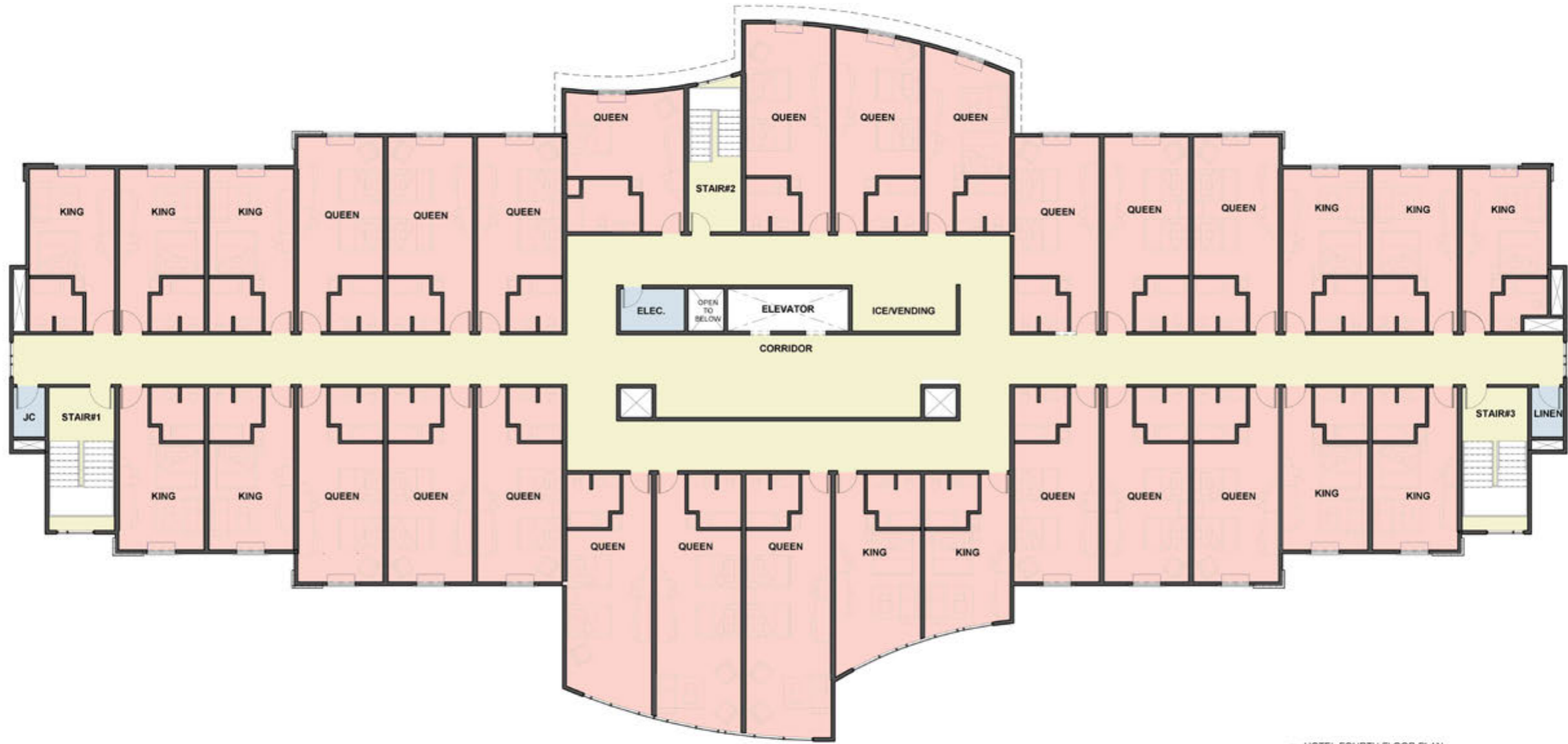
① HOTEL FOURTH FLOOR PLAN
